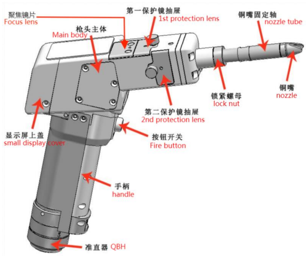
Figure 2.21 Schematic schematic diagram of the gun
