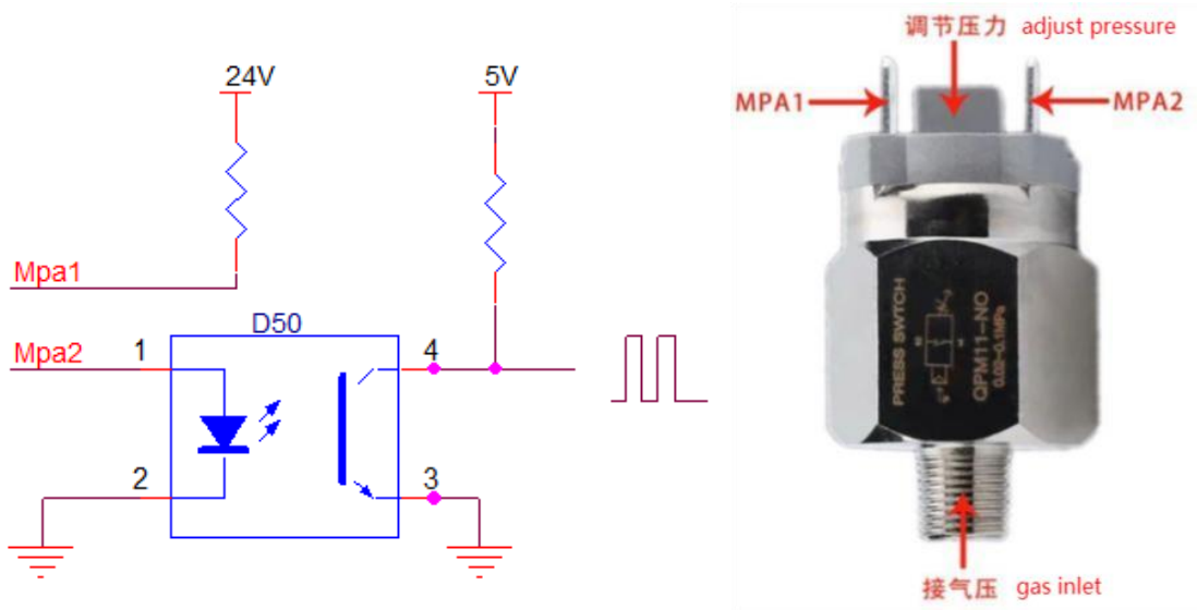
Figure 2.122 Schematic diagram of the air pressure detection interface
