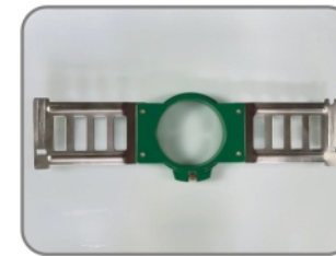
90mm圆框每头2个 Shirt Front Round Hoop 90mm (2pcs/head)
