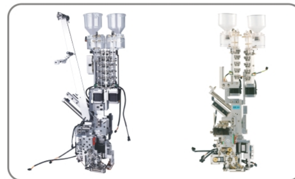
双色珠子加叠金片装置 Twin beads + twin sequin device
