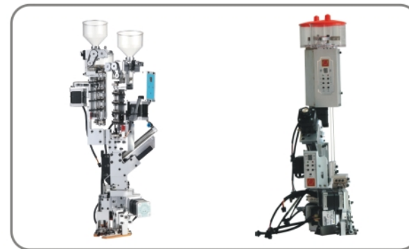
双色珠子装置 Twin beads device
