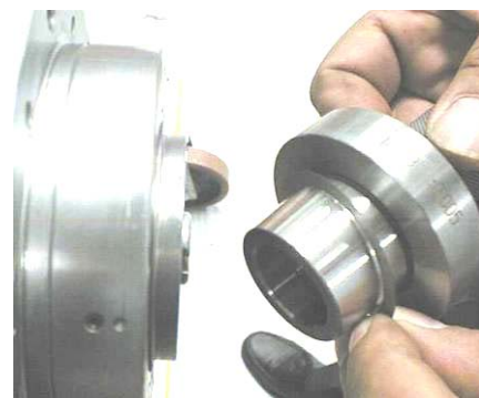
Figure 8.19 interposition of the thickness spacer between the stop surfaces of the gauge and of the spindle shaft
